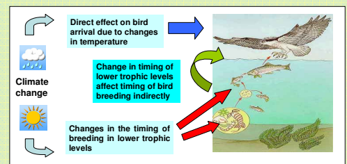
Fig. 1 Phenological changes at different levels of the food chain
